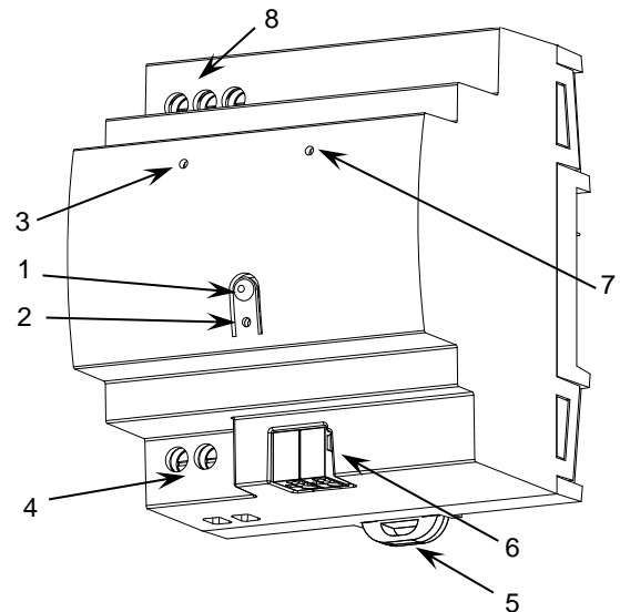
Figure 1: KUPSupply 320mA
